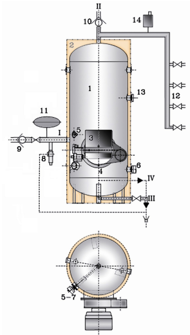
Figure 90.2094.01: Plan indicatif de principe des raccordements
