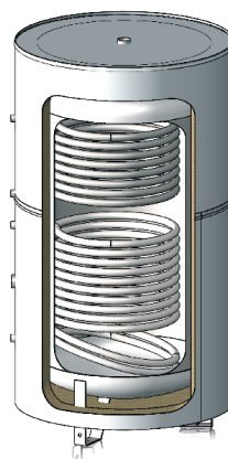
Serpentin(s) Coil(s)
