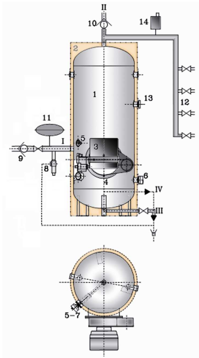
Figure 90.2094.01: Plan indicatif de principe des raccordements
